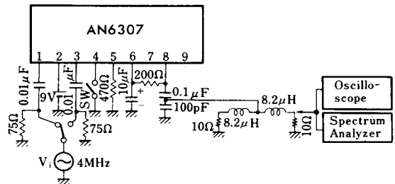
Test Circuit 2 (v o , D 2f , D 3f , CT)
