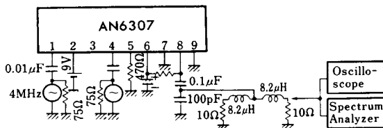
Test Circuit 3 (CM1, CM2)
