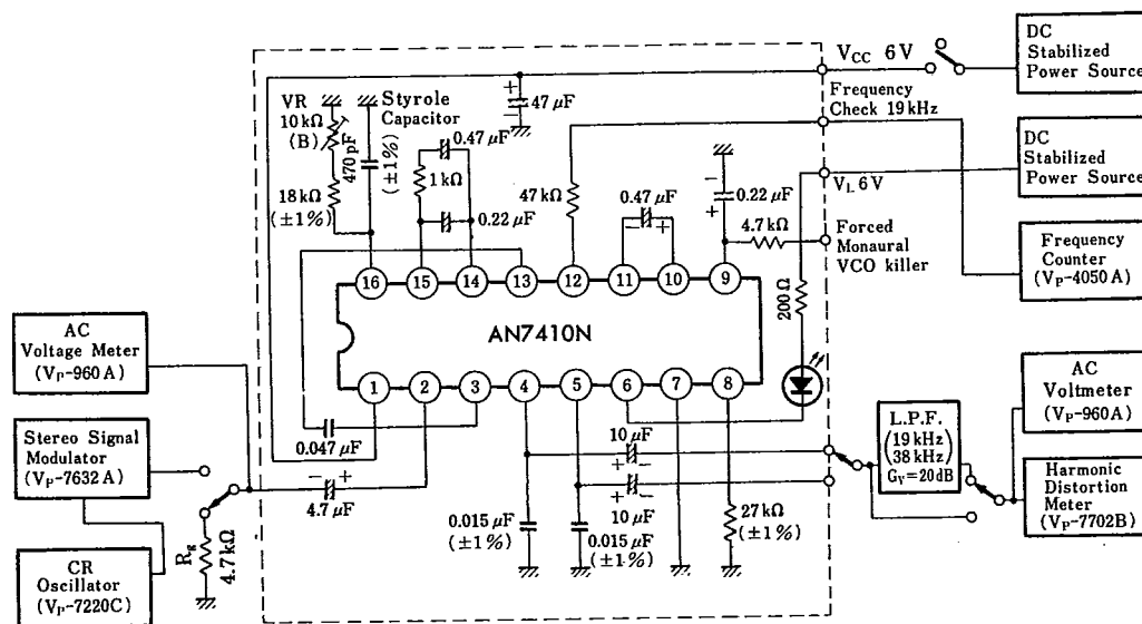
Test Circuit 1
