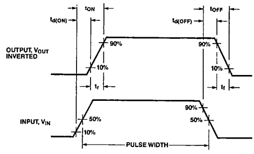
Figure 10 Switching Waveforms
