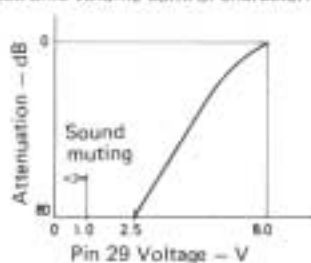
Electronic volume control characteristic
