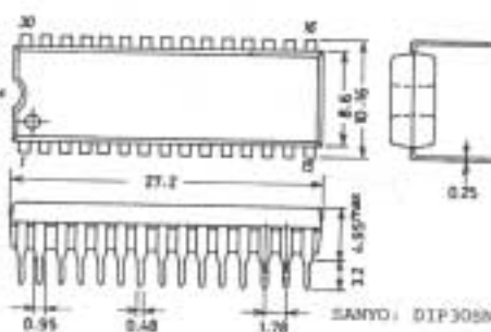
Case Outline 3061-D305NIC (unit : mm)
