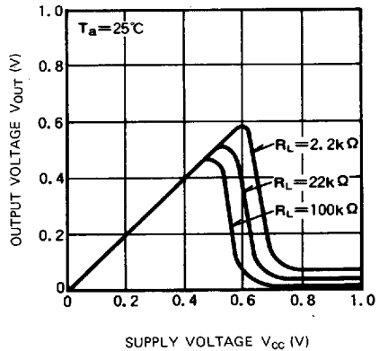
THRESHOLD OPERATING VOLTAGE ([L] reset type)
