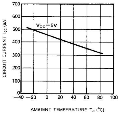
CIRCUIT CURRENT VS. AMBIENT TEMPERATURE (M51953B, M51954B)
