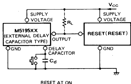
(a) Reset at ON
