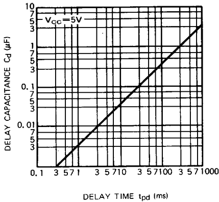
DELAY CAPACITANCE VS. DELAY TIME (M5195XX, External delay capacitor type)
