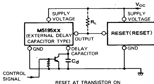
(b) Reset at transistor ON
