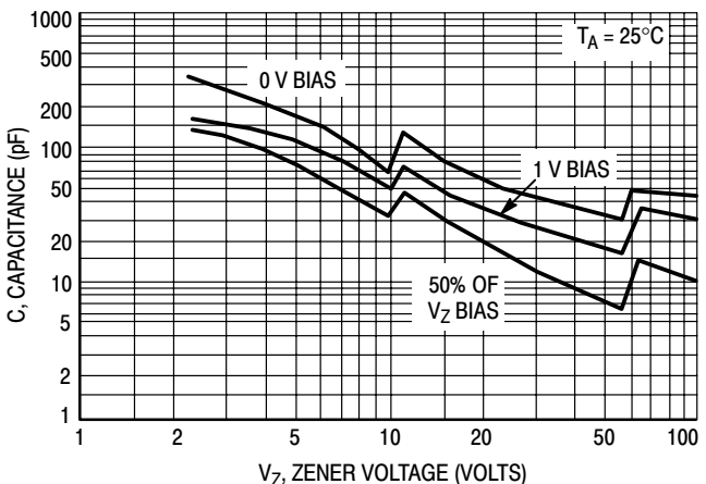
Figure 6a. Typical Capacitance 2-100 Volts
