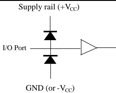
Steering Diode Application
