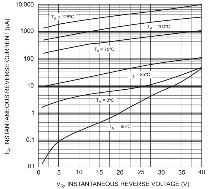
Fig. 6 Typical Reverse Characteristics
