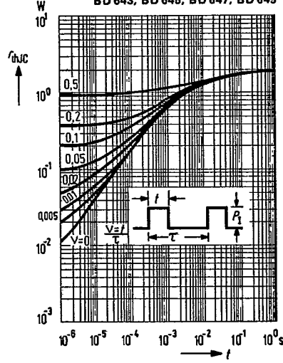
Permissible pulse load r_{thJC} = f(t) ; v = \text{parameter} BD 643, BD 645, BD 647, BD 649
