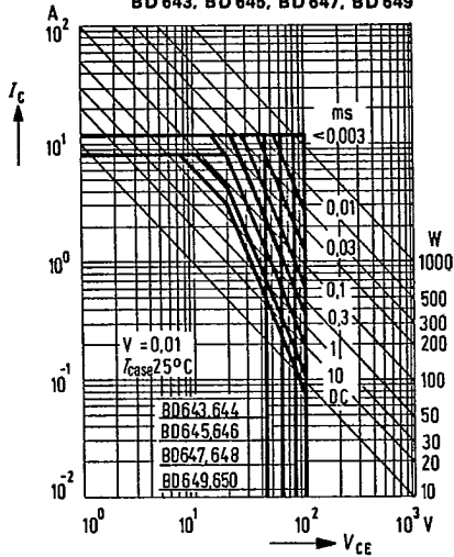
Permissible operating range I_C = f(V_{CE}) ; T_{case} = 25^\circ C , v = 0.01 BD 643, BD 645, BD 647, BD 649
