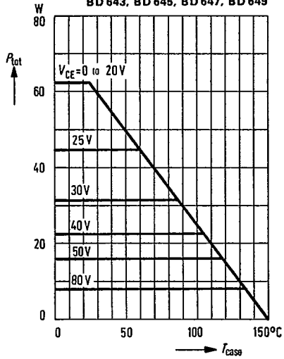
Total perm. power dissipation versus temperature P_{tot} = f(T_{case}) ; V_{CE} = \text{parameter} BD 643, BD 645, BD 647, BD 649
