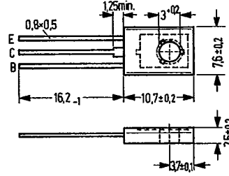
Approx. weight 0.5 g Dimensions in mm
