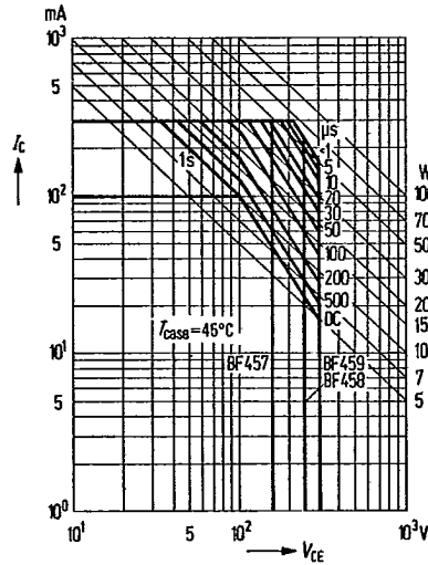
Permissible operating range I_C = f(V_{CE}); (T_{case} = 45^\circ\text{C}); v = 0.1
