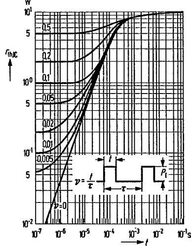
Permissible pulse load r_{thJC} = f(t); v = \text{parameter}
