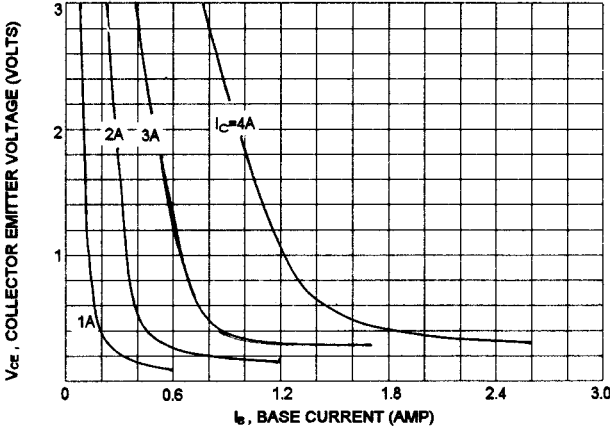
COLLECTOR-EMITTER VOLTAGE
