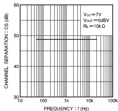
Fig. 7 Channel separation vs. signal frequency
