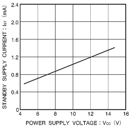
Fig.8 Standby supply current vs. power supply voltage
