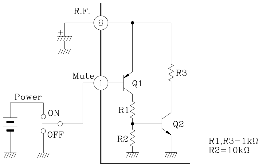
Fig.4 Mute Circuit
