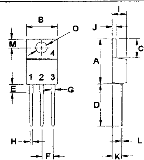
TO-220
