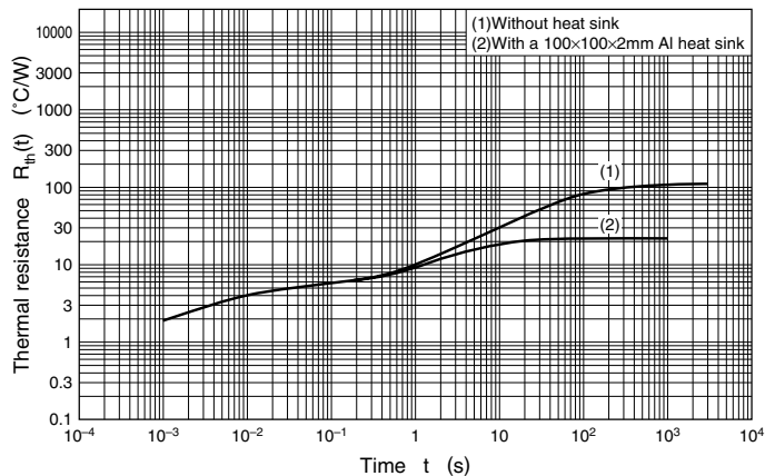
R_{th(t)} - t
