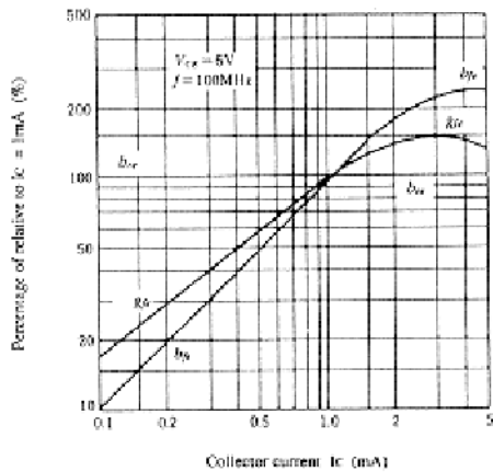
TRANSFER ADMITTANCE VS. COLLECTOR CURRENT
