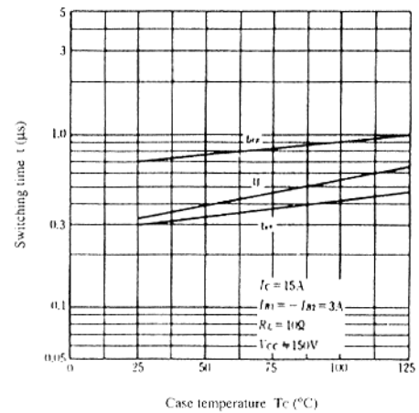
SWITCHING TIME VS. CASE TEMPERATURE
