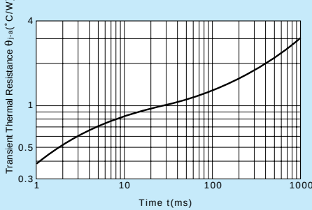
θJA-t Characteristics
