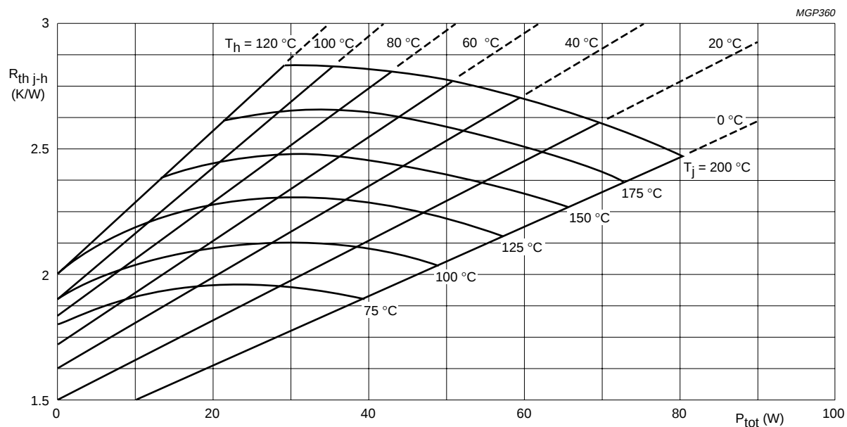
Fig.4 Maximum thermal resistance from junction to heatsink as a function of power dissipation, with heatsink and junction temperature as parameters. ( R_{th\ mb-h} = 0,25 K/W.)
