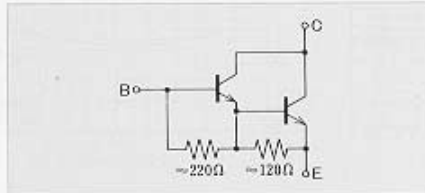
等価回路 Equivalent Circuit
