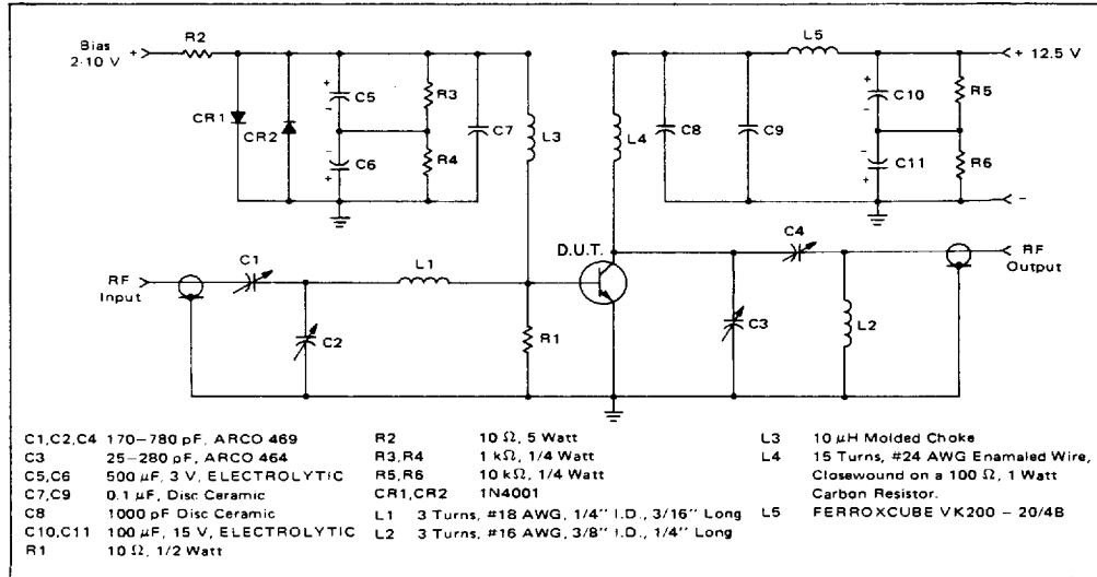
FIGURE 1 - 30 MHz TEST CIRCUIT SCHEMATIC
