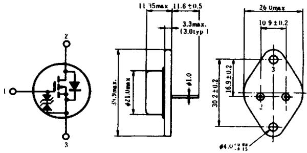
(JEDEC TO-3)
