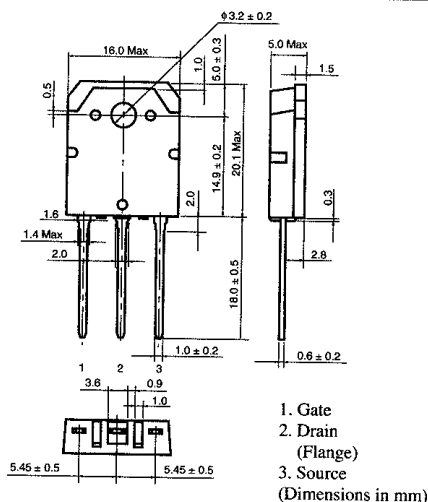
(TO-3P)
