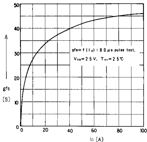
Typical Forward Transconductance vs. I_o
