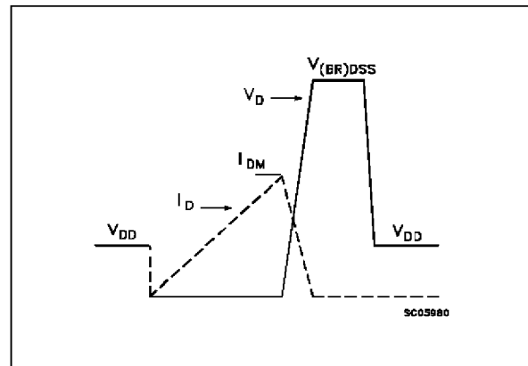
Fig. 2: Unclamped Inductive Waveforms
