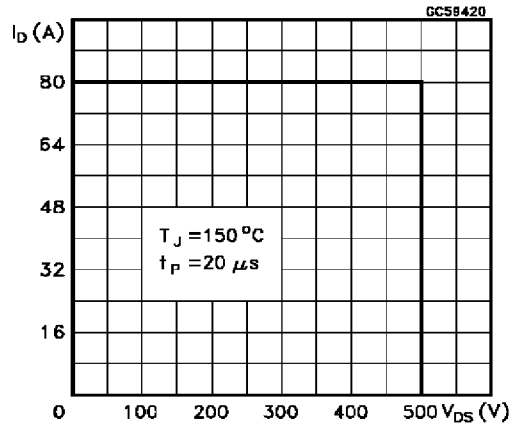
Accidental Overload Area
