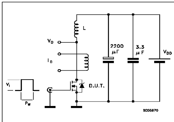
Fig. 1: Unclamped Inductive Load Test Circuits
