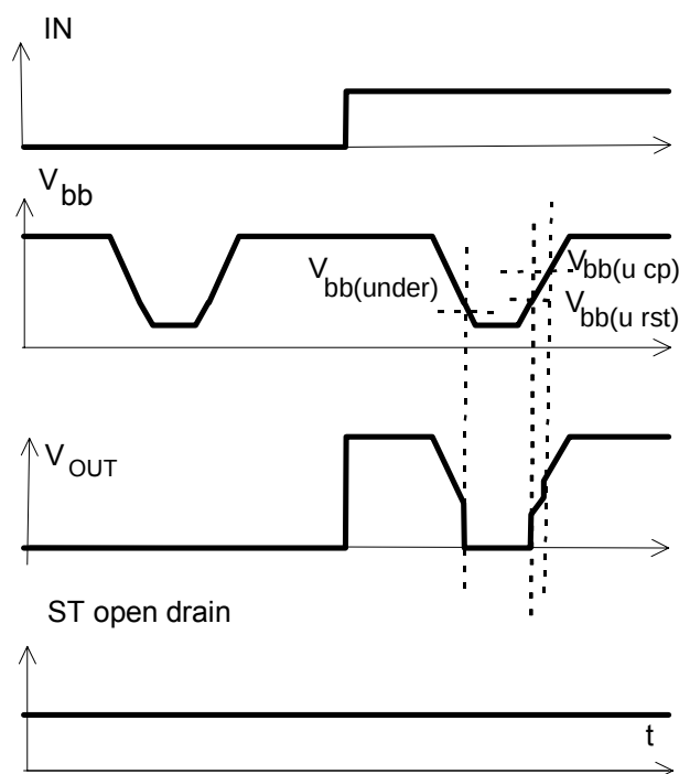
Figure 6a: Undervoltage:
