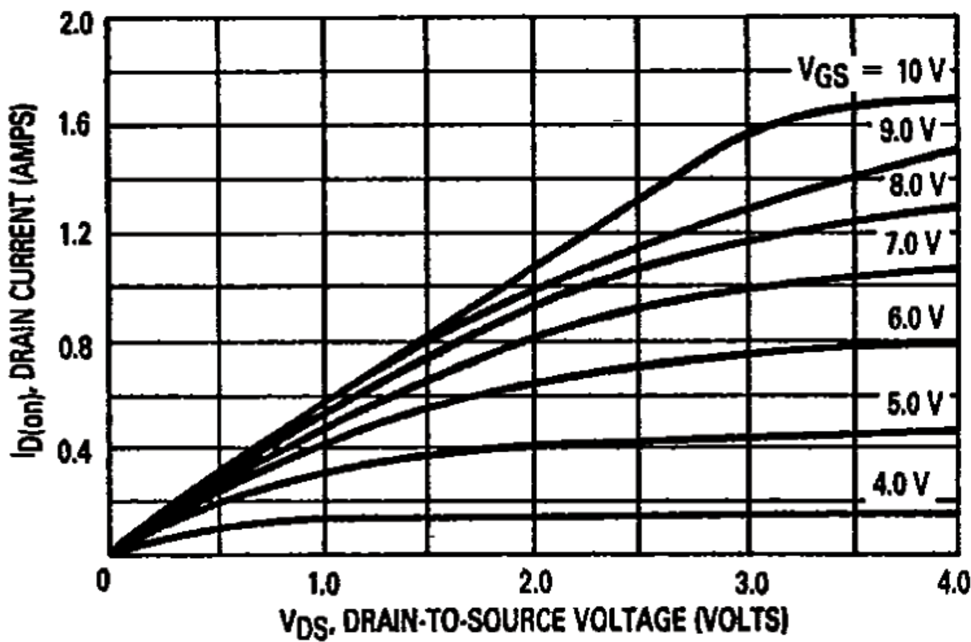
FIGURE 4 — ON-REGION CHARACTERISTICS
