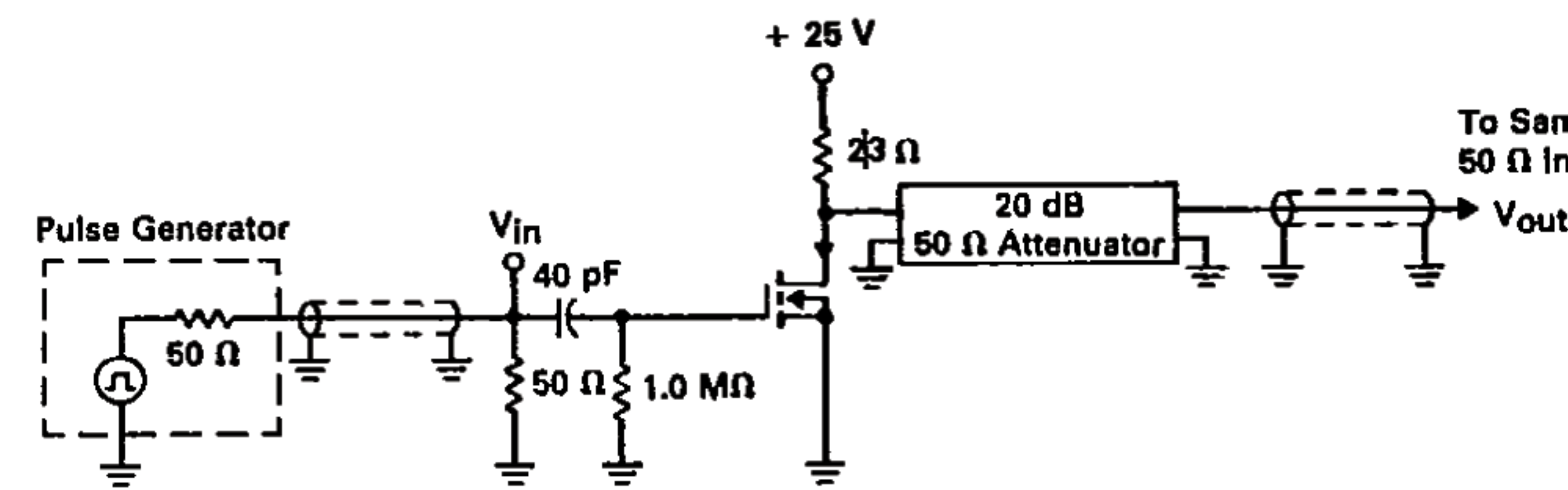
FIGURE 1 — SWITCHING TEST CIRCUIT
