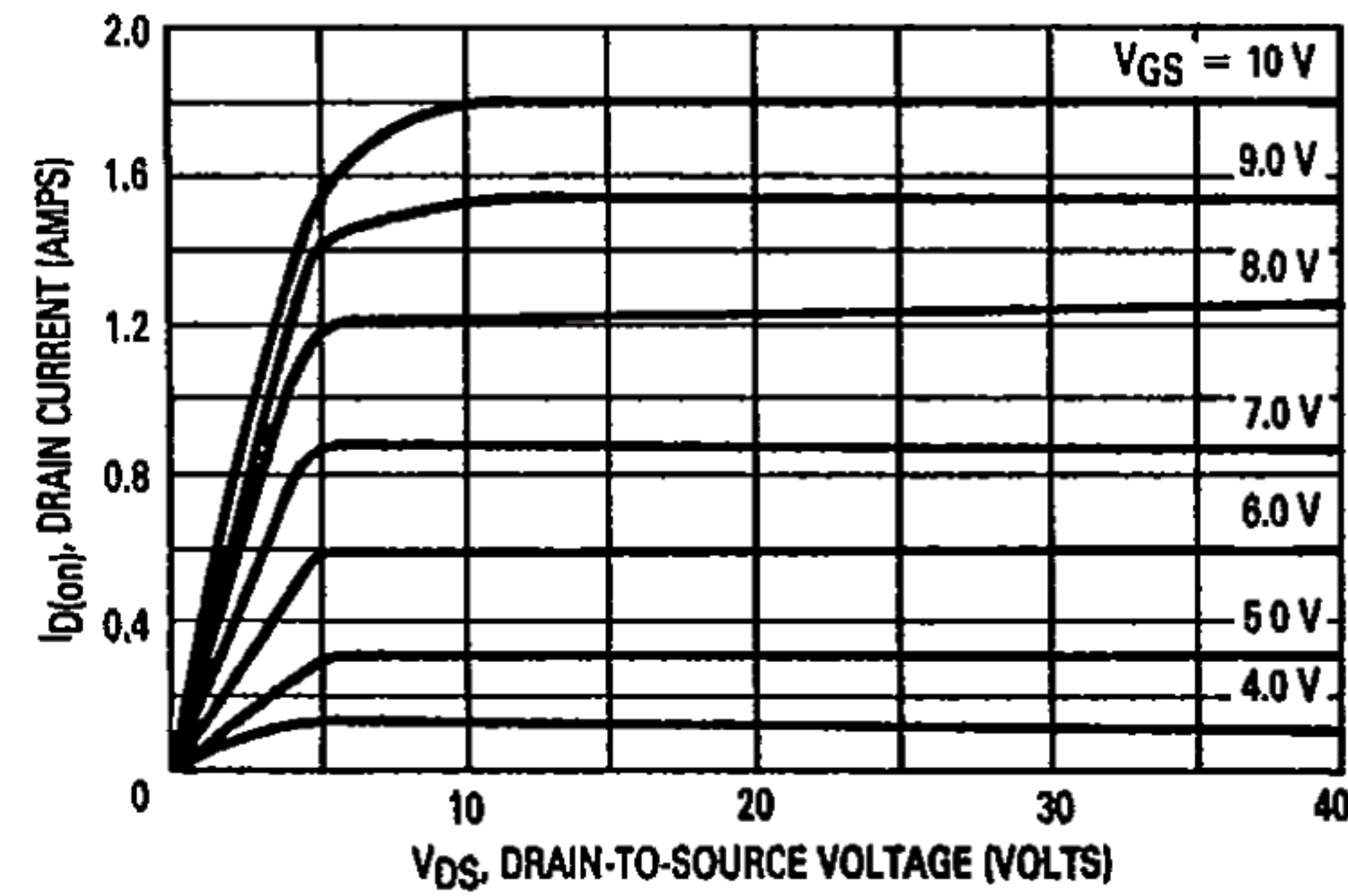
FIGURE 5 — OUTPUT CHARACTERISTICS
