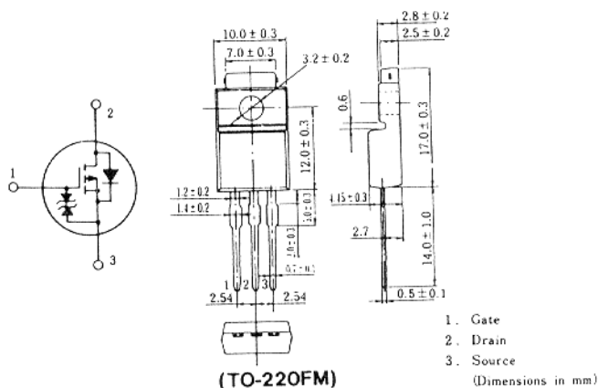
(TO-220FM)
