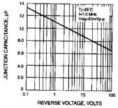
Fig. 6-TYPICAL JUNCTION CAPACITANCE
