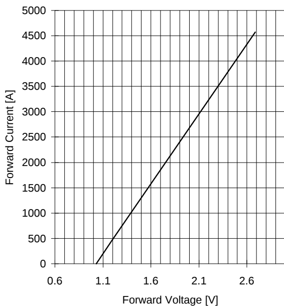
FORWARD CHARACTERISTIC T_j = 150\text{ }^{\circ}\text{C}
