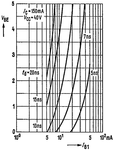
Delay time t_d I_C = 150 \text{ mA}; V_{CC} = 40 \text{ V} BSY 34
