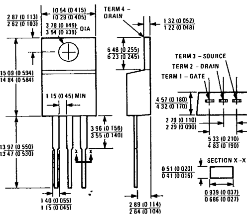
Case Style TO-220AB
