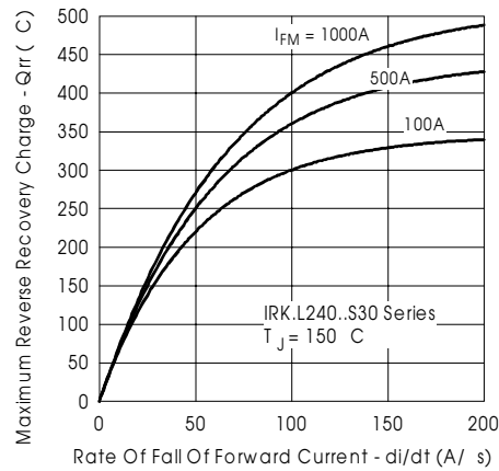
Fig. 19-ReverseRecoveryChargeCharacteristics
