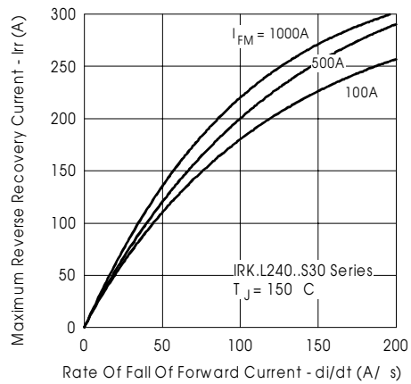
Fig. 20-ReverseRecoveryCurrentCharacteristics
