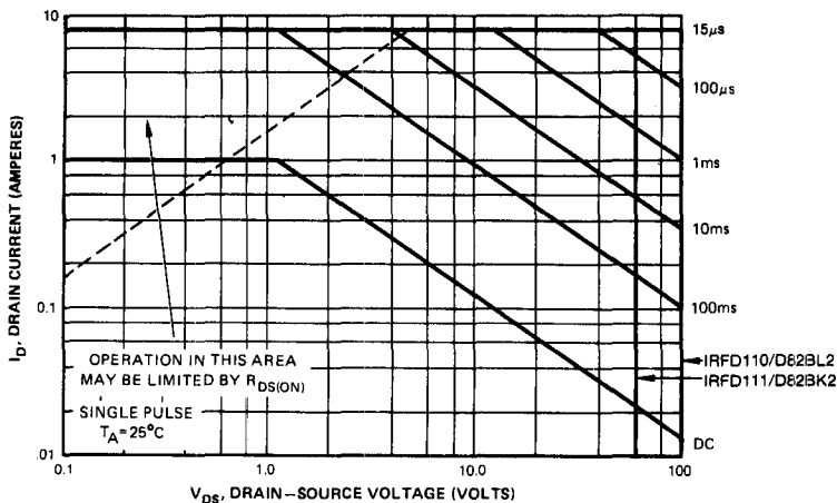
MAXIMUM SAFE OPERATING AREA
