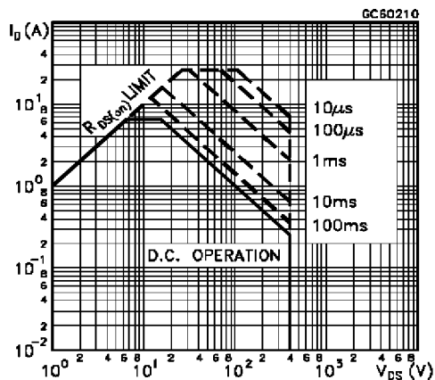
Safe Operating Areas For TO-220
