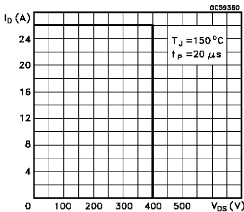
Accidental Overload Area
