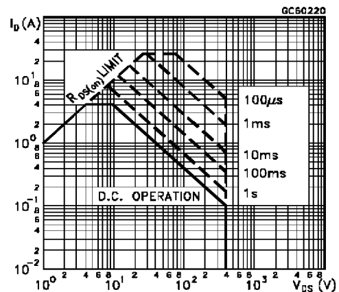
Safe Operating Areas For ISOWATT220
