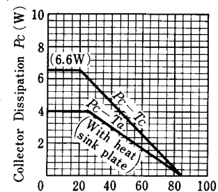
Case Temperature T_C , Ambient Temperature T_a (°C) Maximum Collector Dissipation Curve
