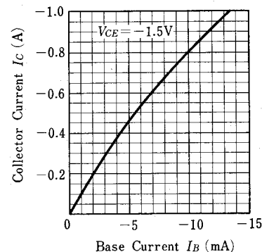
Collector Current vs. Base Current
