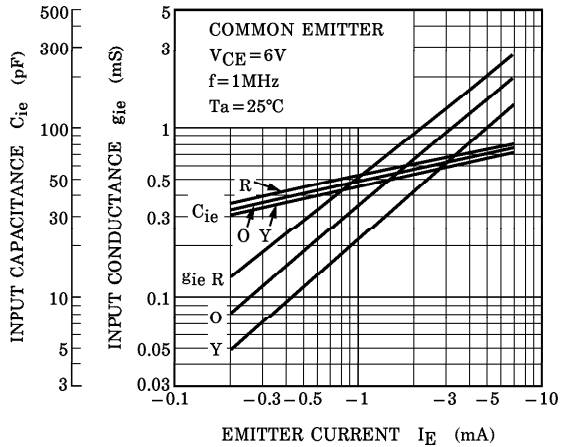
g_{ie}, C_{ie} - I_E
