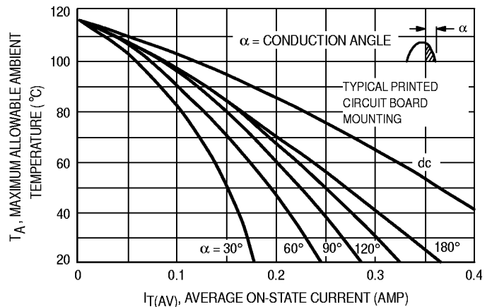
FIGURE 2 – MCR100-8 CURRENT DERATING (REFERENCE: AMBIENT TEMPERATURE)
