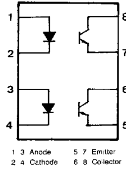
Pin No and internal connection diagram
