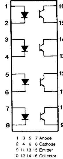
Pin No and internal connection diagram
