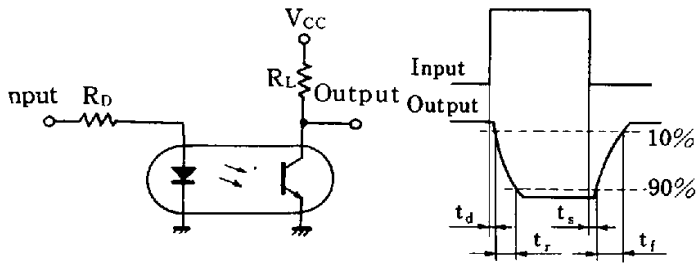
Test Circuit for Response Time
