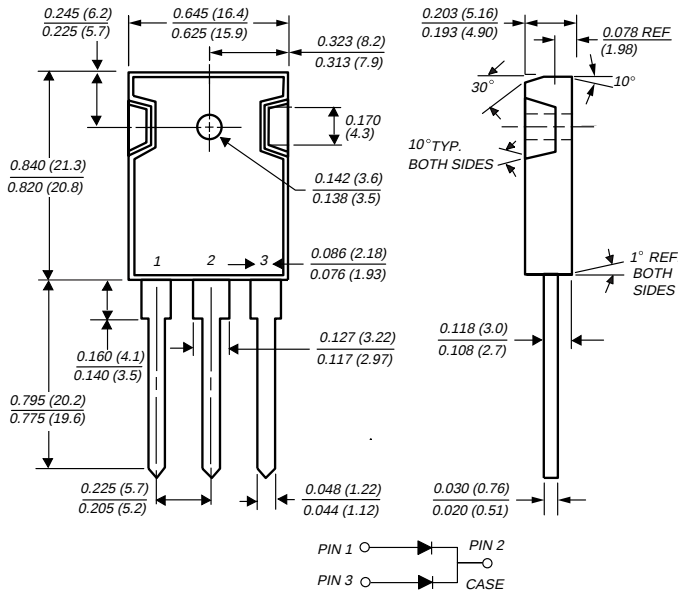
TO-247AD (TO-3P)
