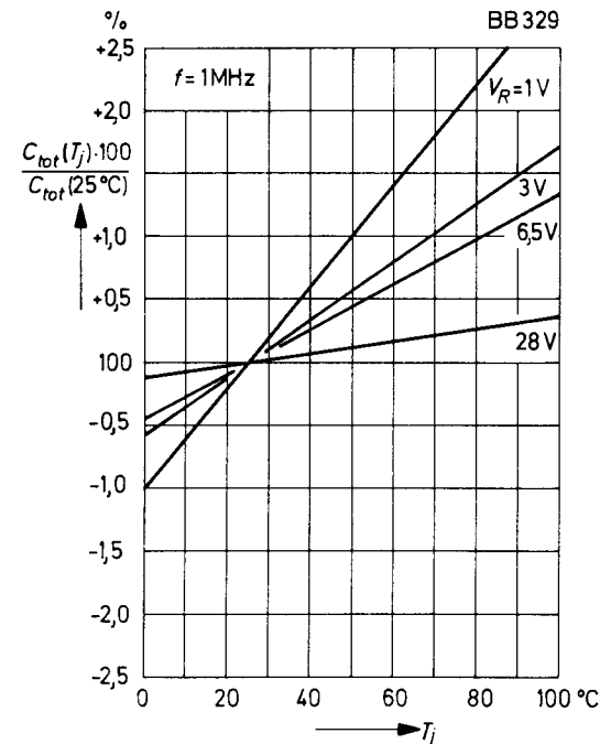
Capacitance versus junction temperature (relative values)
