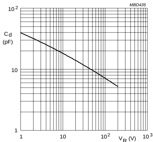
BYM26F and G f = 1\text{ MHz} ; T_j = 25\text{ }^\circ\text{C} .
