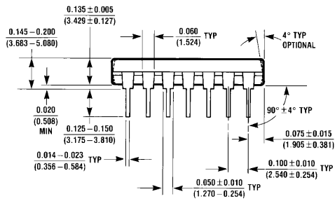
14-Lead Plastic Dual-In-Line Package (N) NS Package Number N14A
