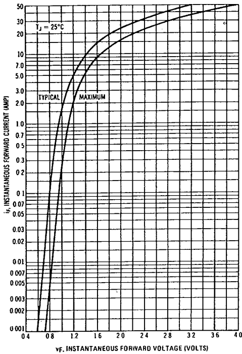
FIGURE 1 - FORWARD VOLTAGE
