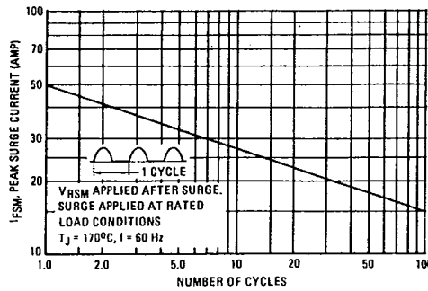
FIGURE 2 - MAXIMUM NONREPETITIVE SURGE CURRENT
