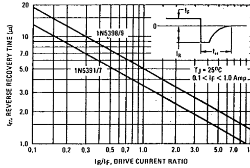
FIGURE 11 - REVERSE RECOVERY TIME
