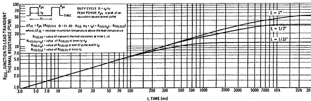
FIGURE 4 - TYPICAL TRANSIENT THERMAL RESISTANCE
