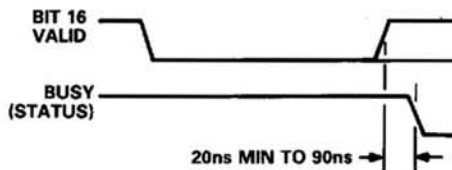
Figure 9. LSB Valid to Status Low
