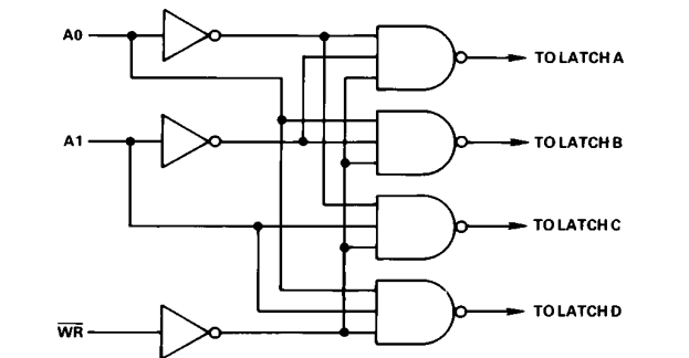
Figure 4. Input Control Logic
