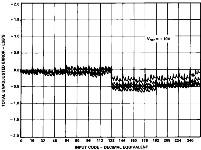
Figure 6. Channel-to-Channel Matching
