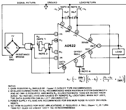
Figure 1. Typical Bridge Application
