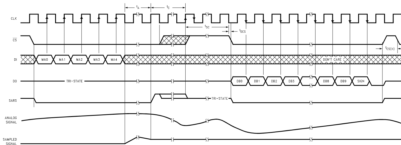
FIGURE 11. ADC10732, ADC10734 and ADC10738 Using \overline{CS} to Delay Output of Data after a Conversion has Completed
