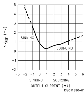
Load Regulation
