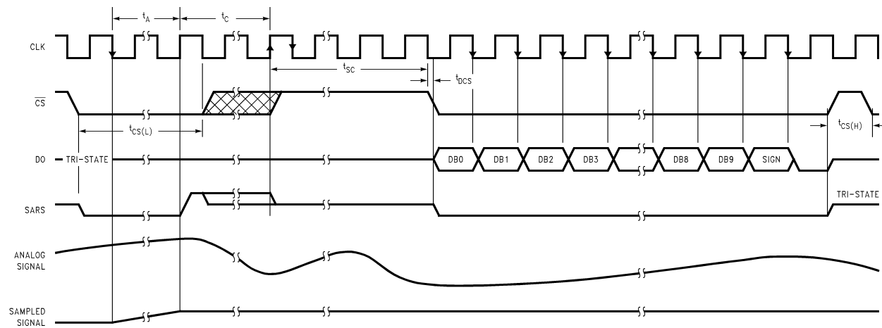
FIGURE 10. ADC10731 Using \overline{CS} to Delay Output of Data after a Conversion has Completed
