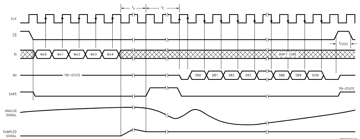
FIGURE 9. ADC10732, ADC10734 and ADC10738 \overline{CS} Low during Conversion
