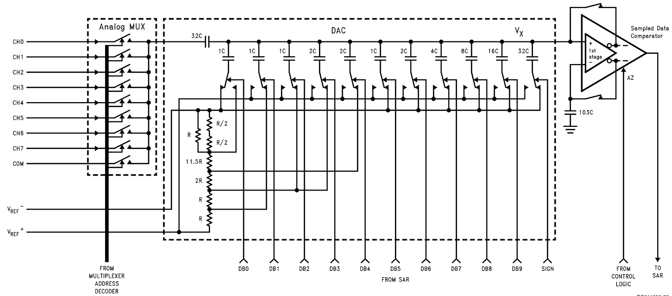
FIGURE 12. Detailed Diagram of the ADC10738 DAC and Analog Multiplexer Stages
