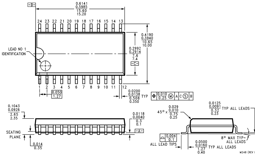
Order Number ADC10738CIWM NS Package Number M24B
