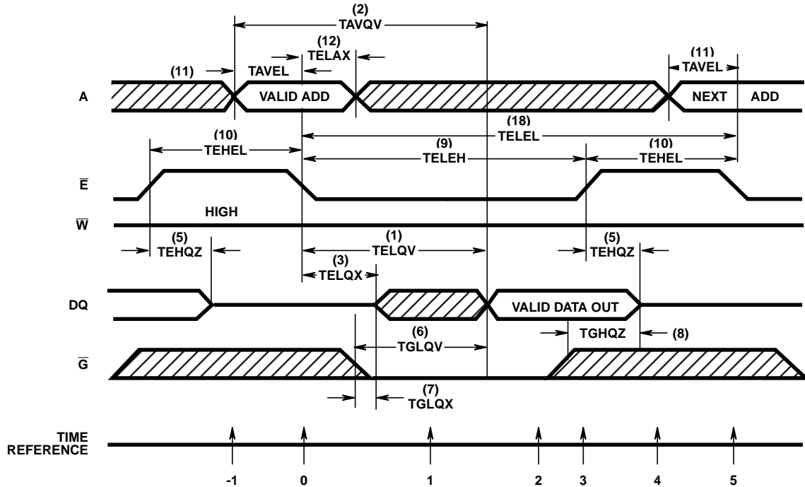
FIGURE 1. READ CYCLE
